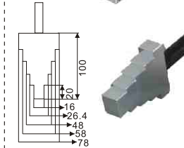
SWRSB1 安全墊塊 Safety Block
